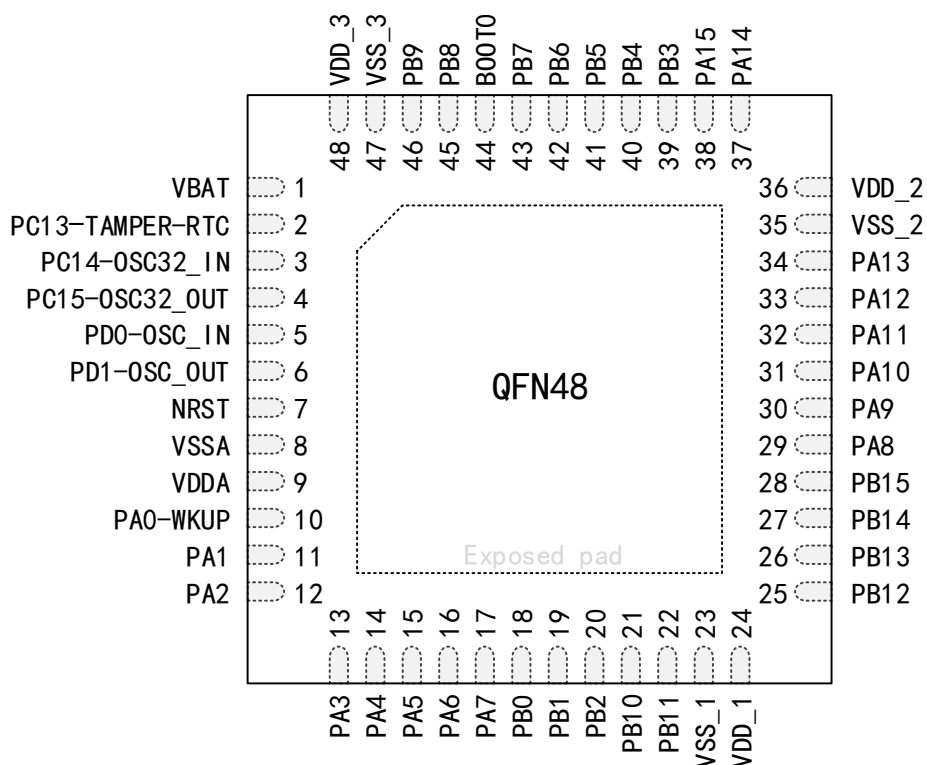
Figure 3 Distribution Diagram of APM32F403xB Series QFN48 Pins
