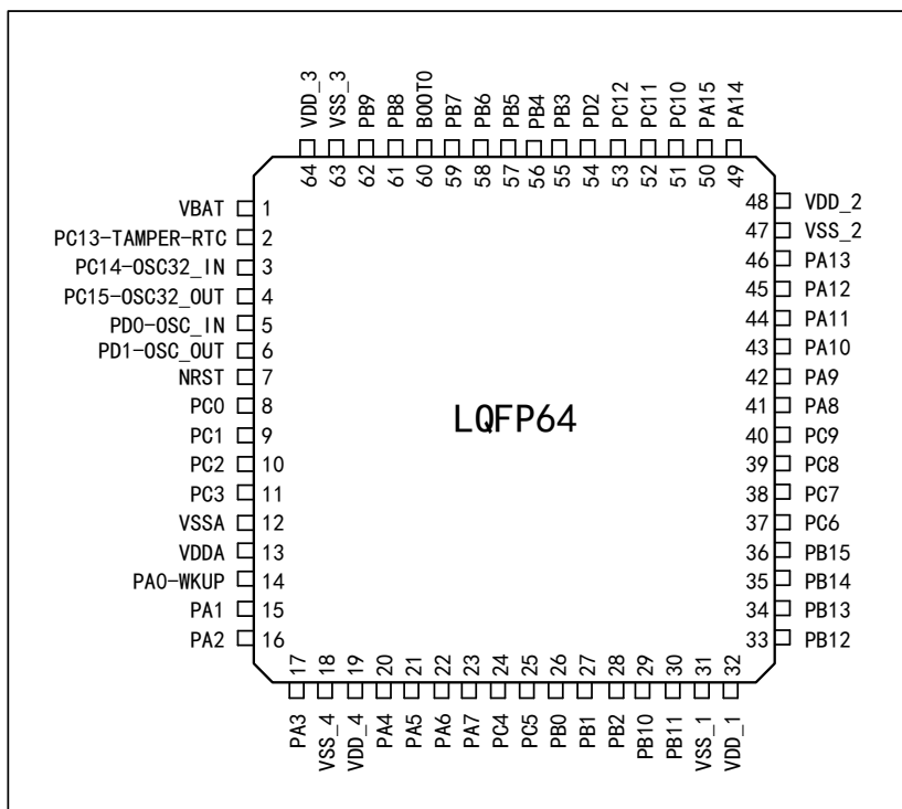
Figure 1 Distribution Diagram of APM32F403xB Series LQFP64 Pins
