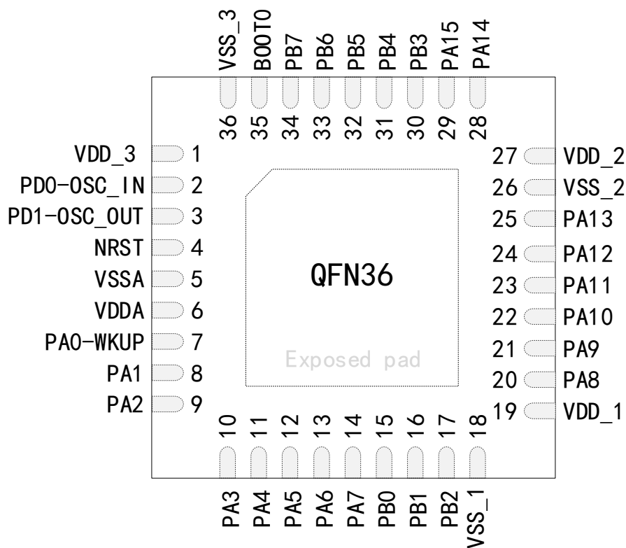
Figure4 Distribution Diagram of APM32F403xB Series QFN36 Pins
