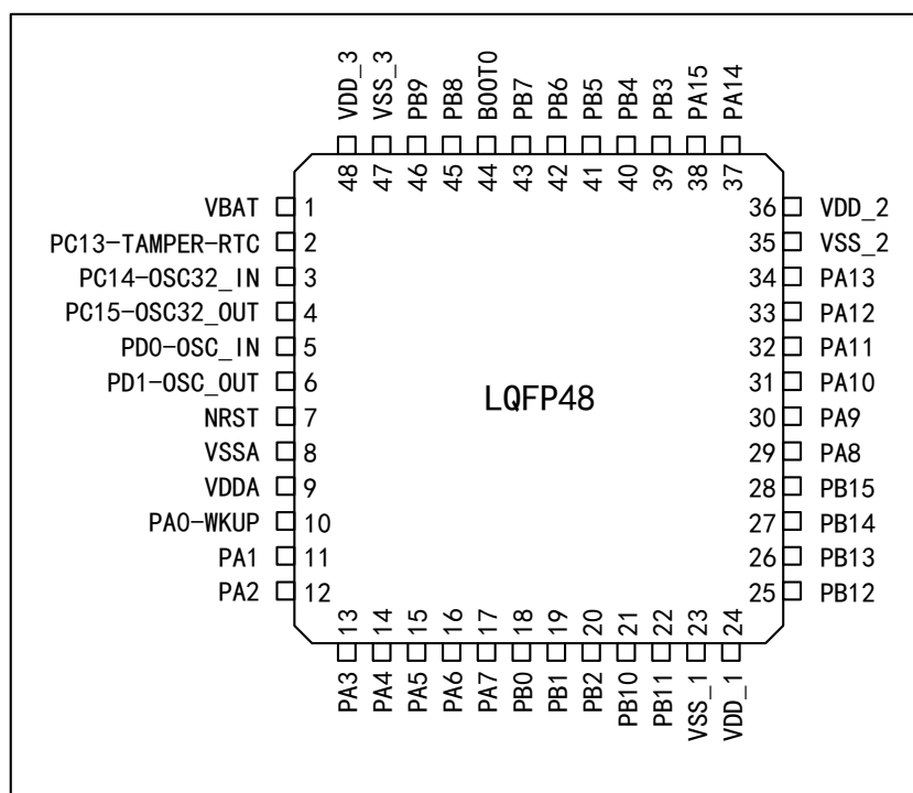
Figure 2 Distribution Diagram of APM32F403xB Series LQFP48 Pins
