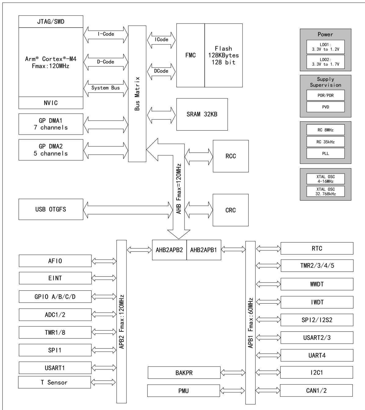
Figure 5 APM32F403xB System Block Diagram
