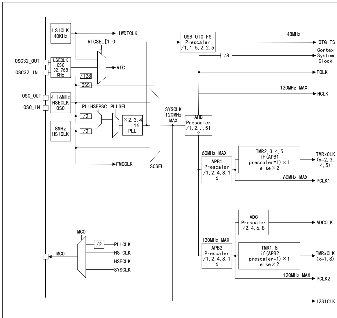
Figure 6 APM32F403xB Clock Tree
